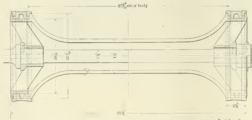
PISTON VALVES—INSIDE ADMISSION—4-4-2 PENNSYLVANIA LINES.
